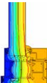
➤ C70S OPEN-IN / TBT THERMAL PROFILE
