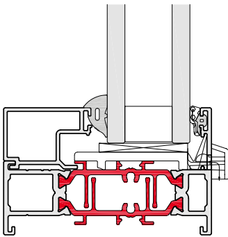
➤ C70S OPEN-IN FRAME DETAIL
