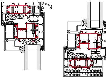
➤ C70S OPEN-OUT FRAME AND VENT DETAIL
